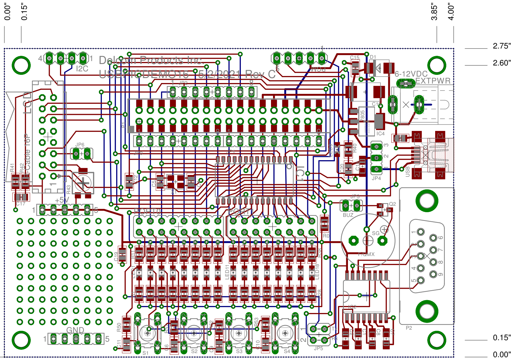
Delcom Products Inc. USB PICDEMO16 5/2/2021 Rev C
